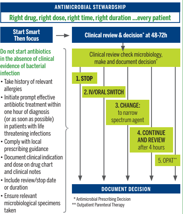
Figure 20: Antimicrobial Stewardship Treatment Algorithm
