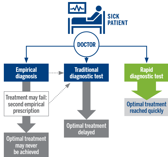
Figure 23: How rapid diagnostic tests help optimize treatment
